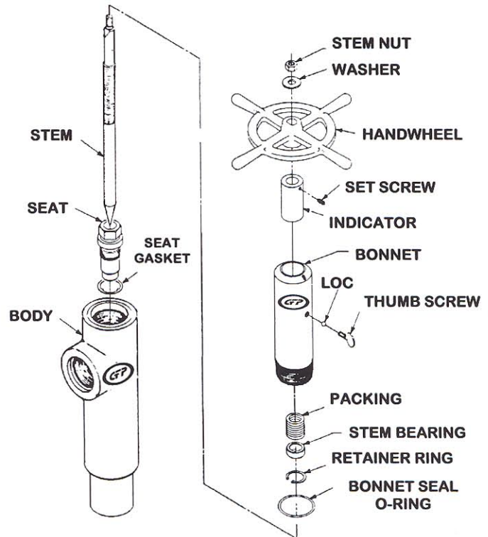
Typical Threaded Long Nose Heater Choke
